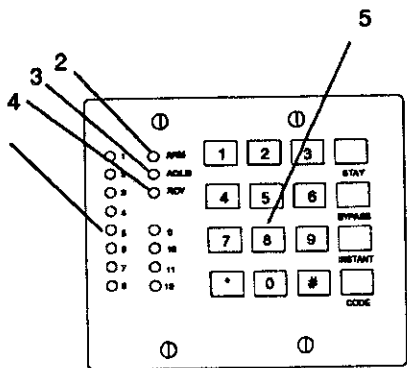
XL4612RM KEYPAD
